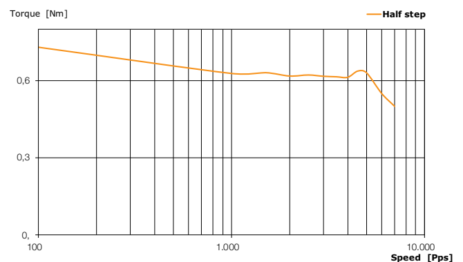
57STC41-4204AC VM: 24V; 4,2A/Phase Driver: SMD 103
